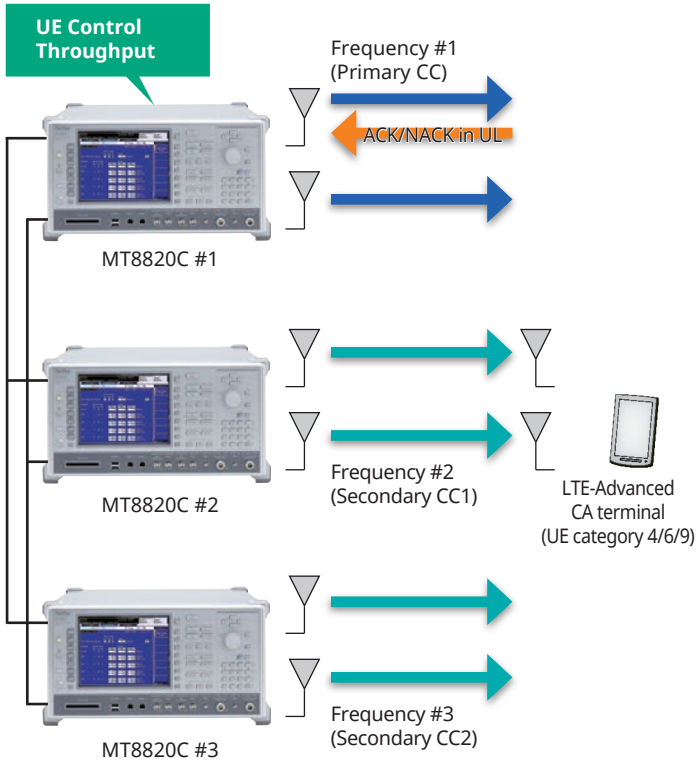
Example of MT8820C Connection (2x2 MIMO)
