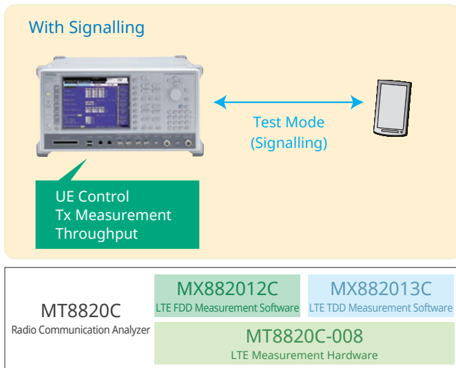
Example of LTE FDD and TDD configuration
