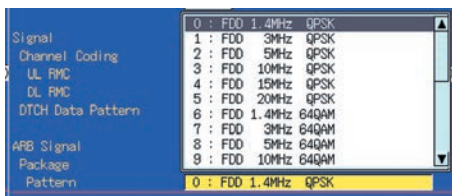
DL Signal Pattern (LTE FDD)
